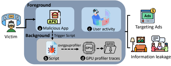
Fig. 1: Illustration of OVRWATCHER's threat model.
